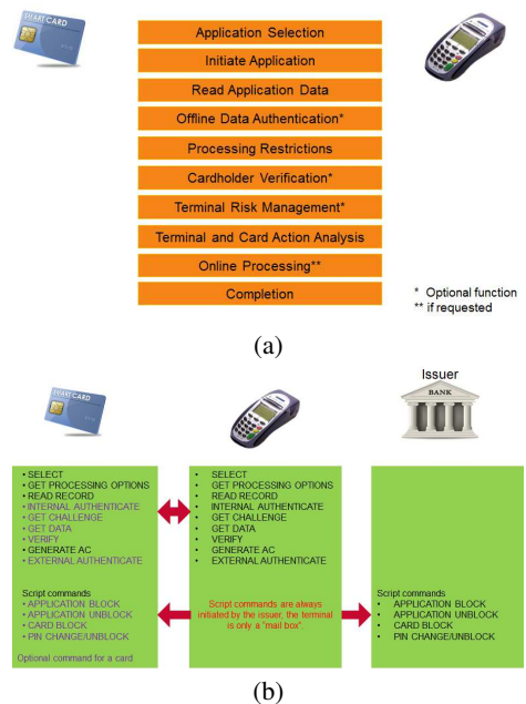
Fig. 1. (a) Transaction flow, (b) Command library
